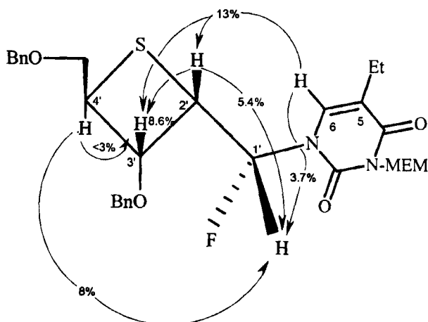
FIGURE: nOe enhancements ( \rightarrow ) in thietane (23)
